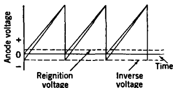
FIG. 8-47.—Anode-voltage waveform with and without inverse voltage.
